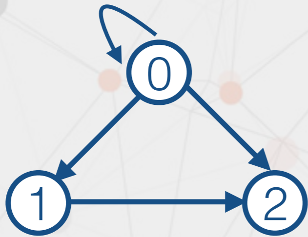
Graph with a self edge
